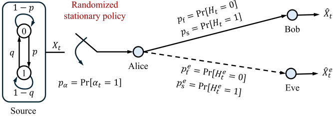
Fig. 1. Remote reconstruction system over a wiretap channel with a transmitter (Alice), a legitimate receiver (Bob), and an eavesdropper (Eve).
